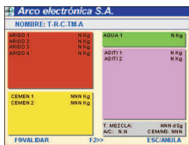
PANTALLA TFT 5-7" / 5-7" TFT SCREEN
